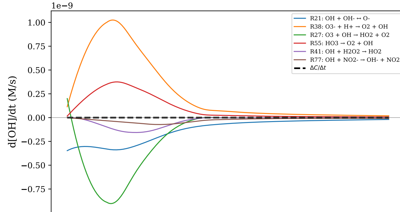
(b) OH [final=0.05 pM]
