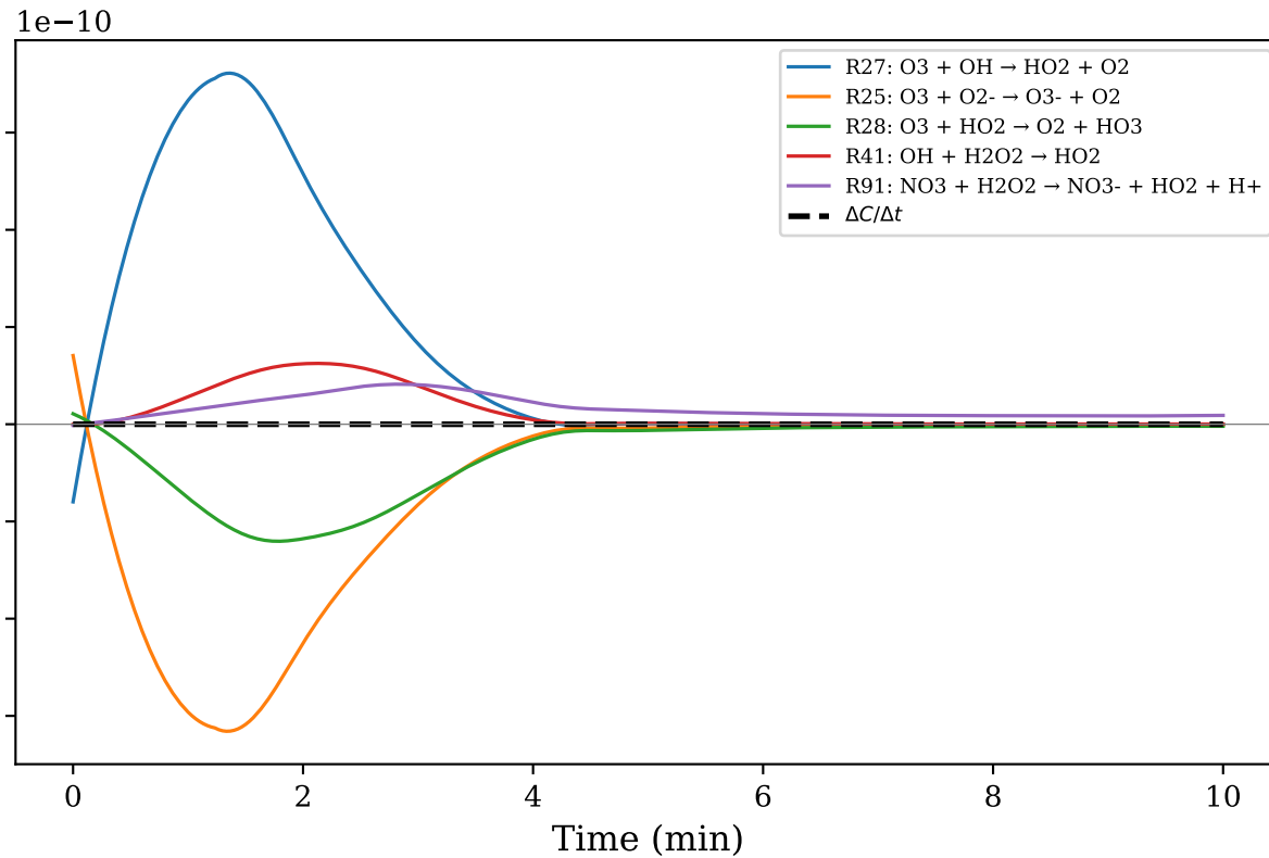
(c) HO 2 [final=1.68 pM]
